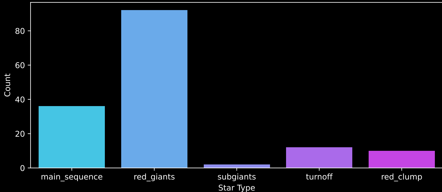
APOGEE DR17 Field: [348+17-O] Count plot of Star Type
