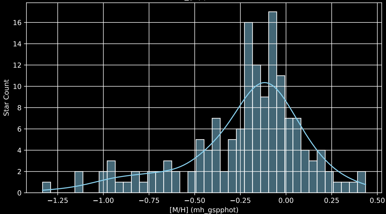
APOGEE DR17 Field: [348+17-O [M/H] (mh_gspphot) (n= 150)
