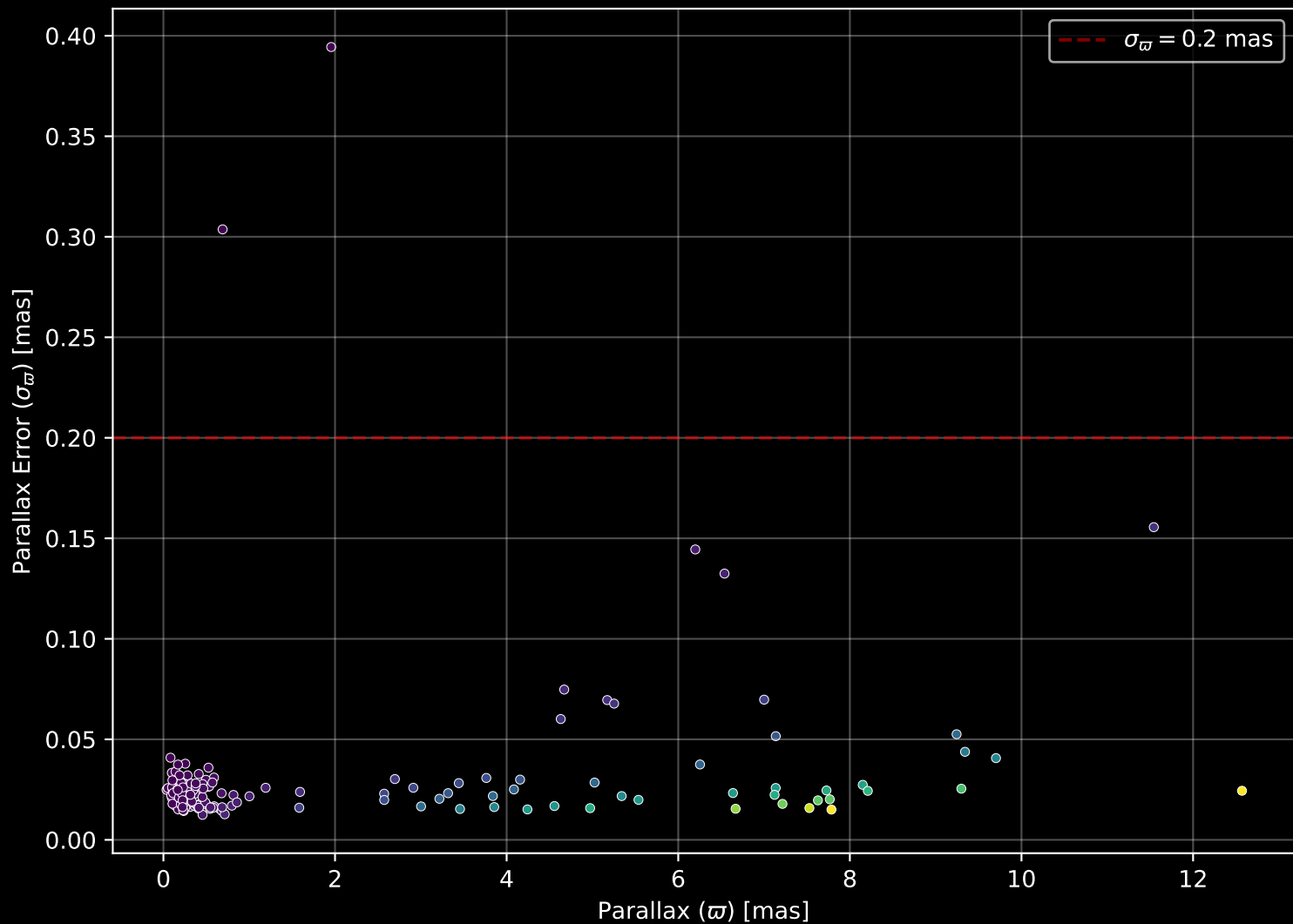
APOGEE DR17 Field: [348+17-O] Parallax Quality (n= 152)
