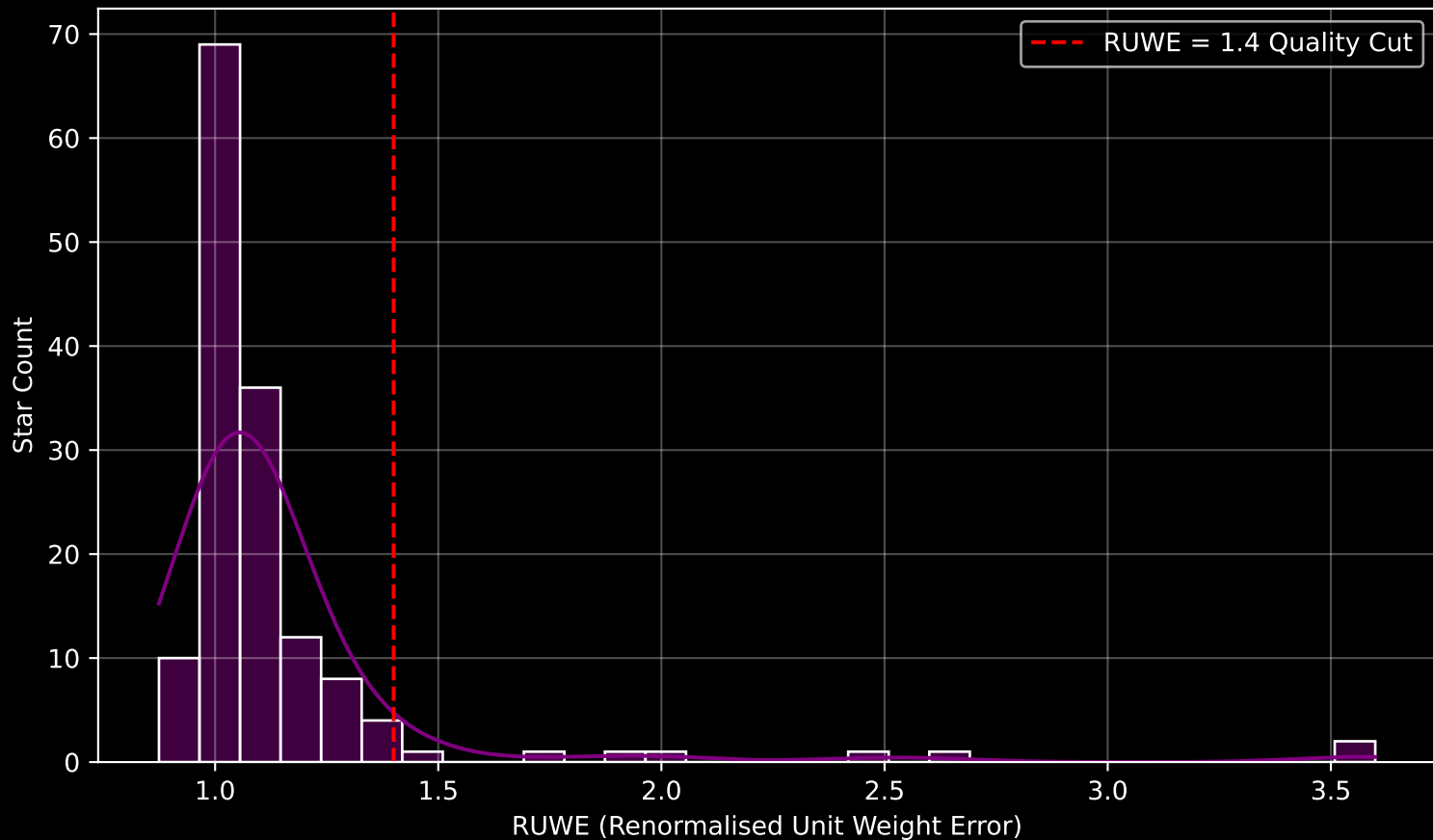
GAPOGEE DR17 Field [348+17-O] RUWE Distribution (n= 147)
