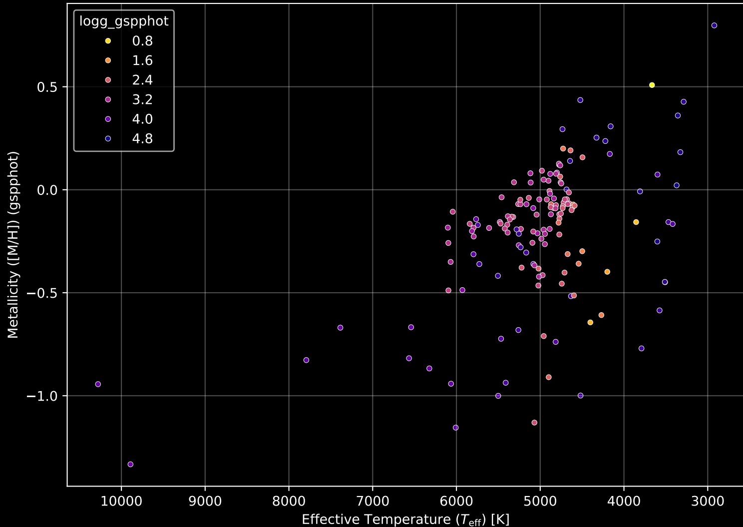
APOGEE DR17 Field: [348+17-O] Stellar Population Parameters (n= 152)
