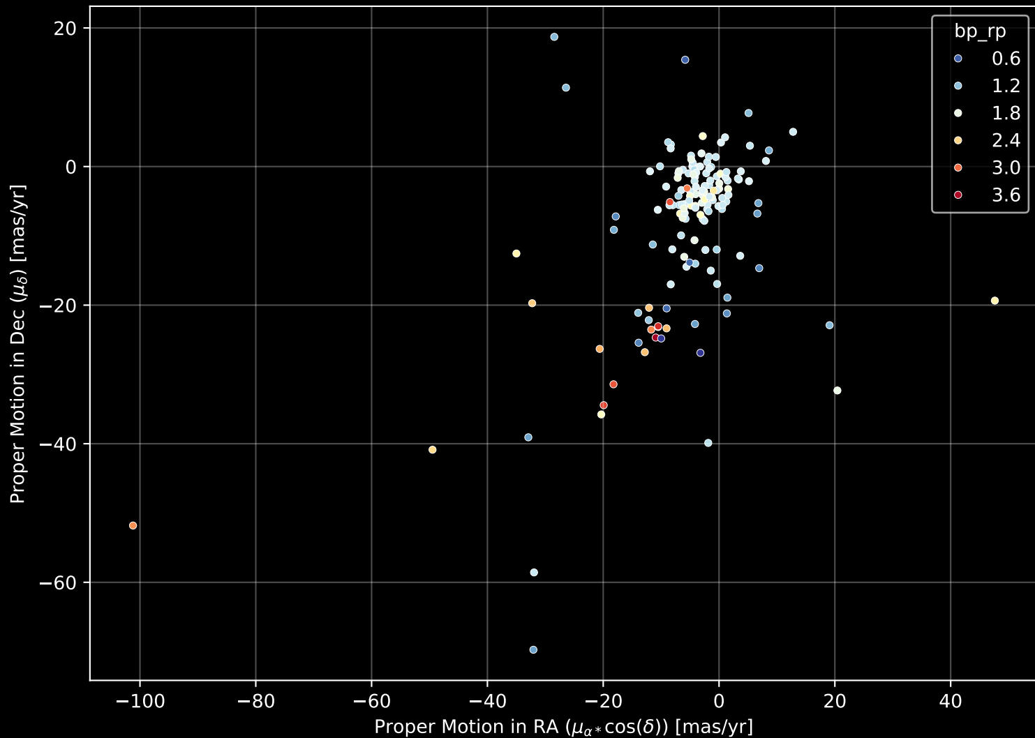
APOGEE DR17 Field: [348+17-O] Proper Motion Diagram (n= 152)
