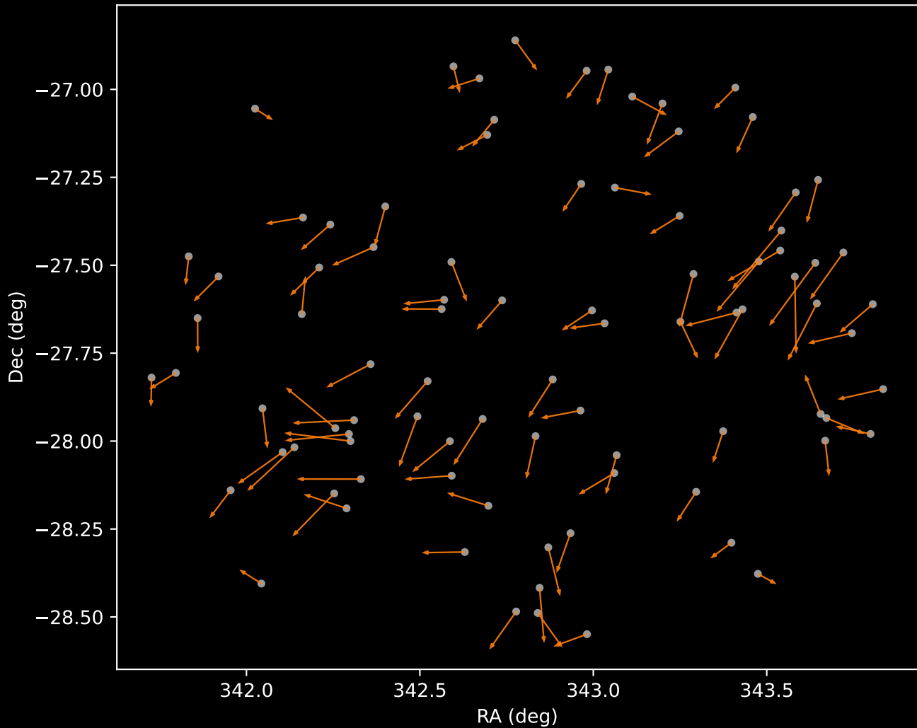
APOGEE DR17 Cluster 2 Proper Motion Vectors (n=88)
